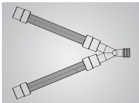
16044 Patient breathing circuit kit, 48"
